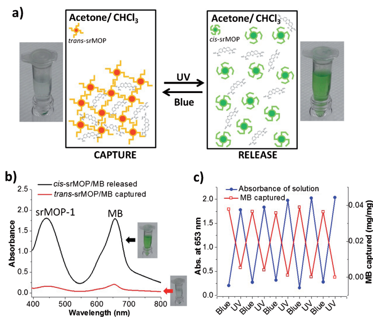
Figure 4. a) Schematic illustration of the reversible formation of insoluble trans -srMOP-1 and soluble cis -srMOP-1, which enable the photoinduced capture and release of MB, respectively. The left photograph shows the clear supernatant with insoluble MB@ trans -srMOP-1 at the bottom after centrifugation at 15 000 rpm. The right photograph shows a homogeneous solution of cis -srMOP-1 and MB. b) UV/Vis spectra of a solution of srMOP-1 and MB after UV irradiation (black) as well as after irradiation with blue light (red). c) Absorbance of the solution at 653 nm (blue) and the corresponding concentration of MB captured in srMOP-1 (red).
